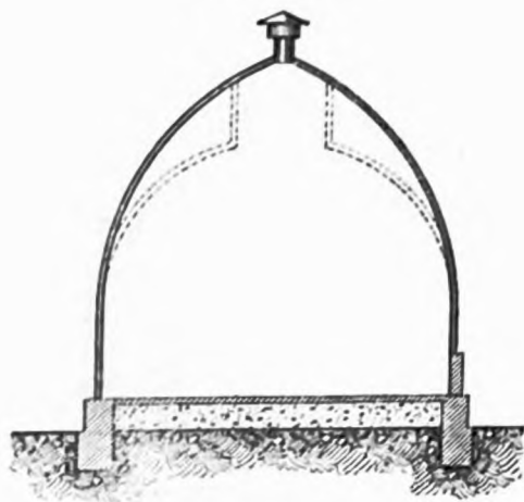
Tollet's Pavillontypus.
