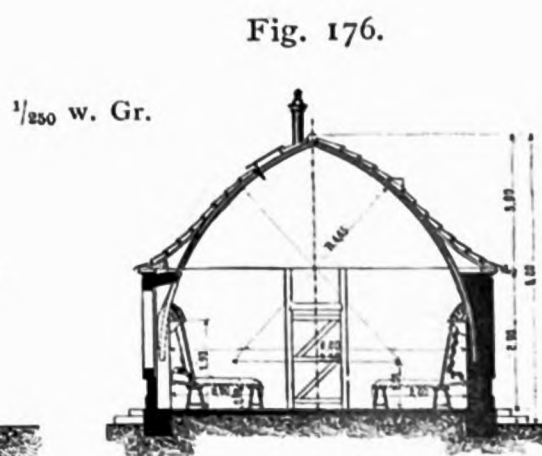
Tollet's Lagerpavillon.
