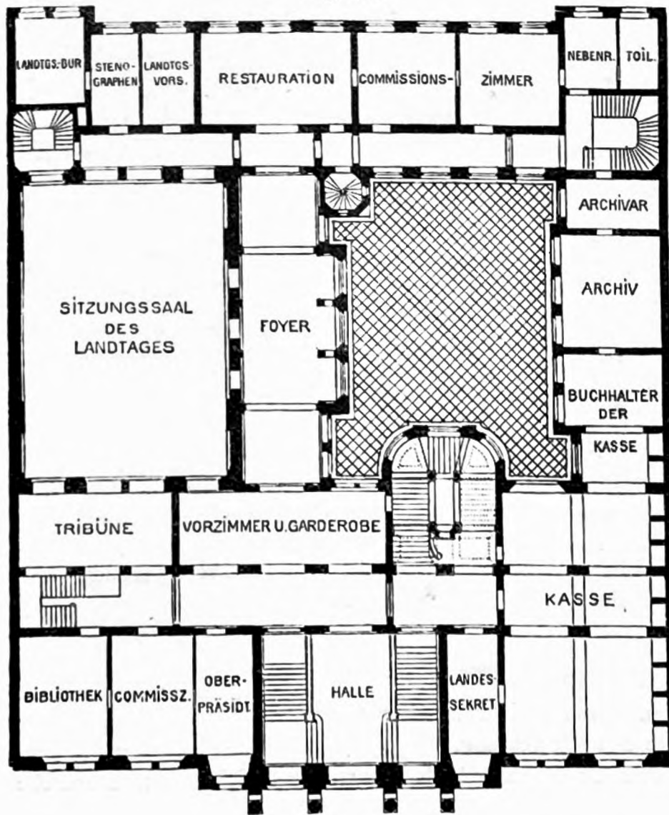
Erdgeschoss.
