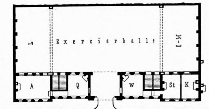
Exerzierhaus zu Shoreditch. Erdgeschoss. — \frac{1}{500} w. Gr. Arch.: Higgins.
